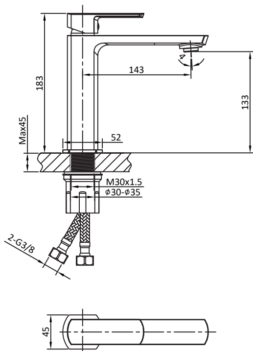
Installation drawing
